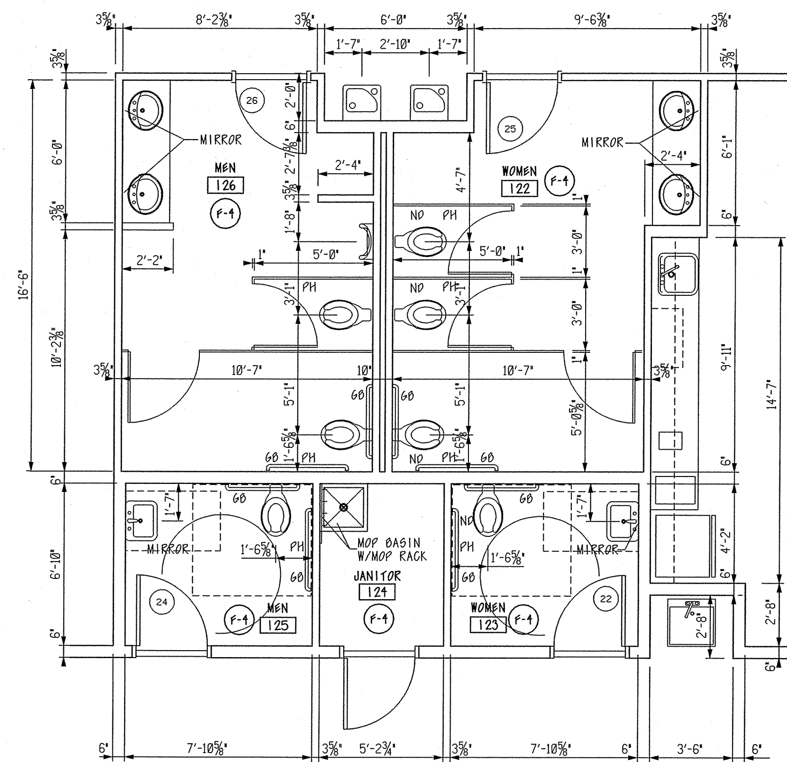
LARGE SCALE PLAN
