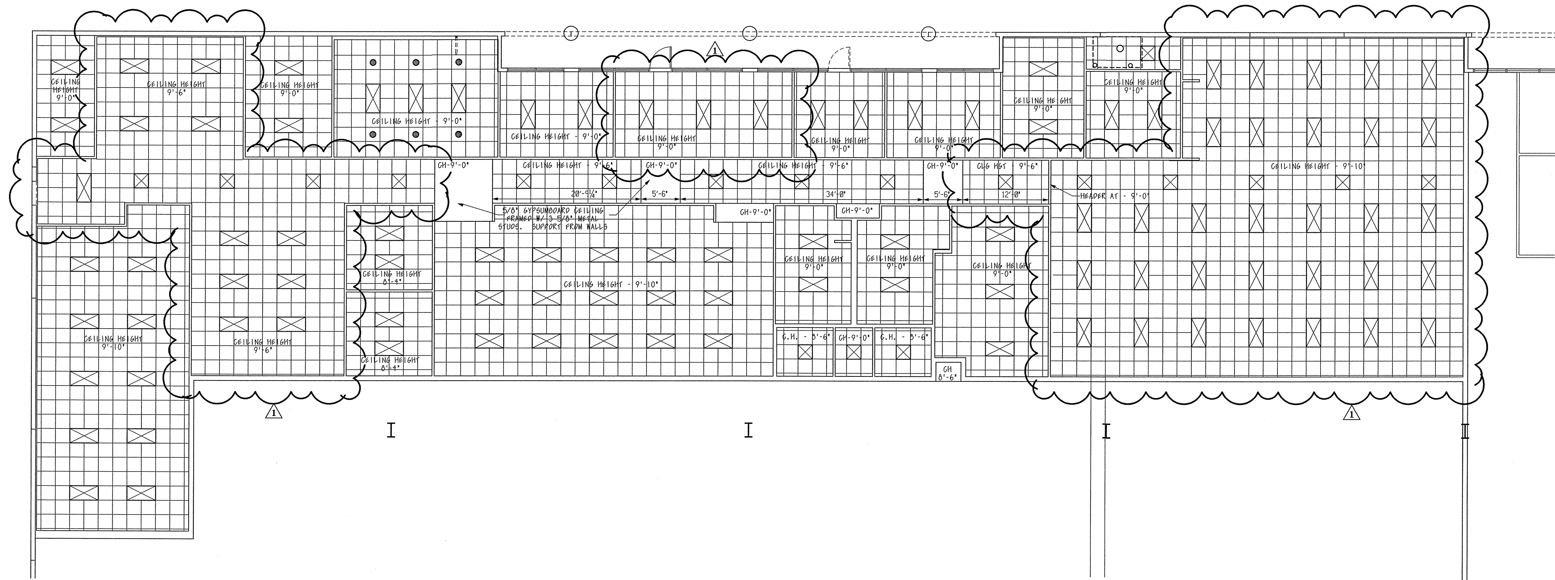
CEILING PLAN
