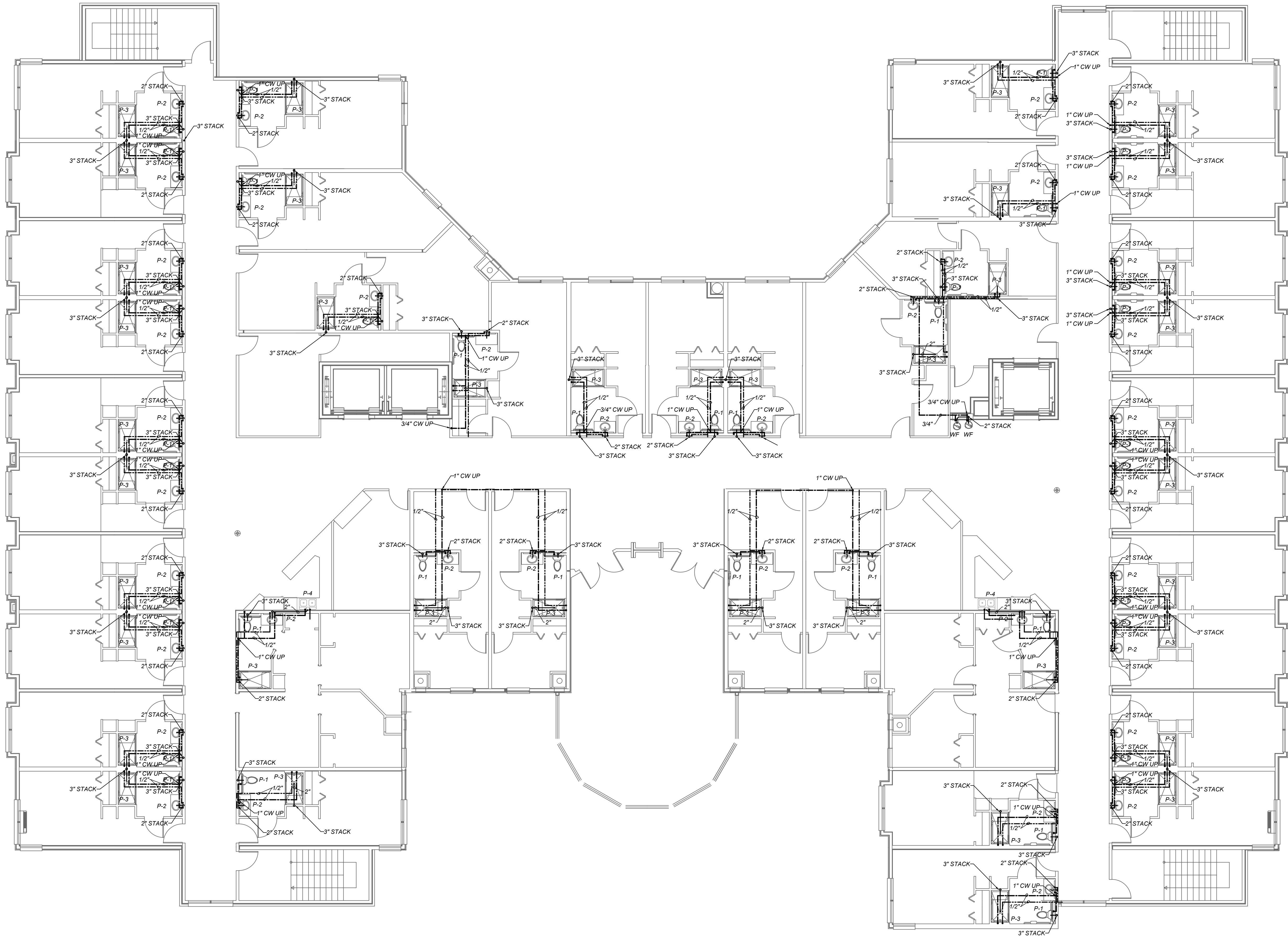
1 P6 3RD FLOOR PLUMBING PLAN 1/8"=1'
