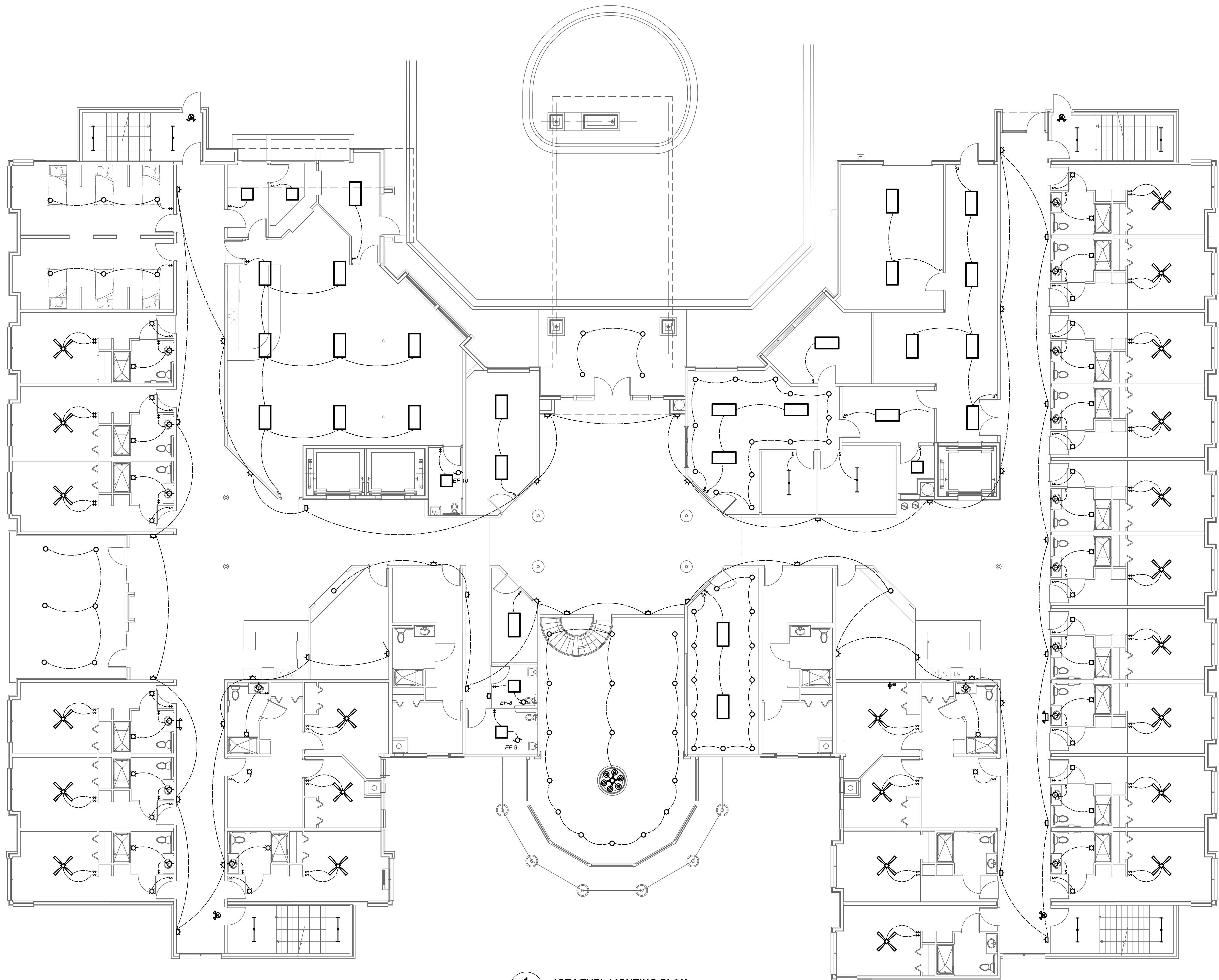
1 E9 1ST LEVEL LIGHTING PLAN 1/8"=1'
