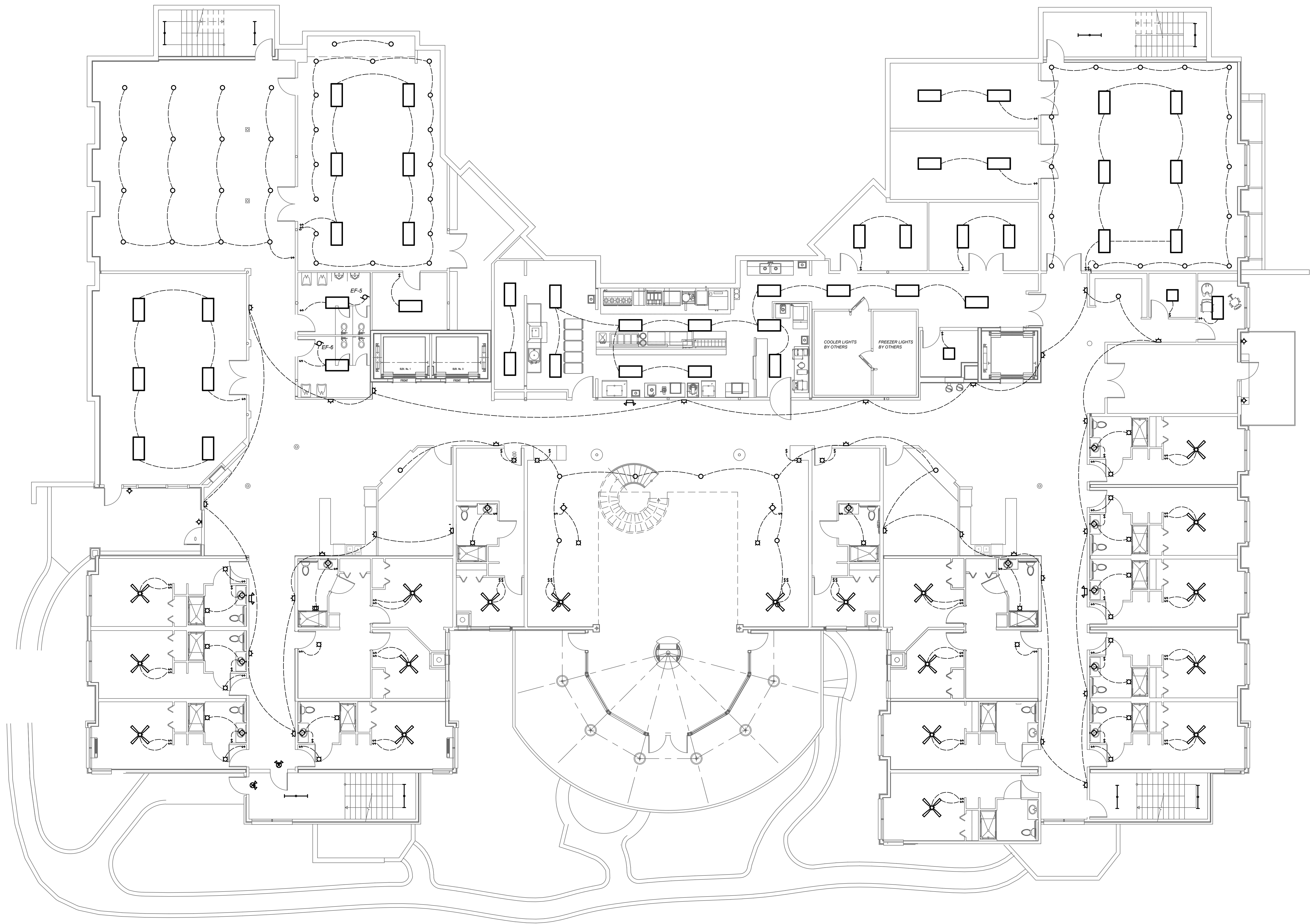
1 PATIO LEVEL LIGHTING PLAN E8 1/8"=1'
