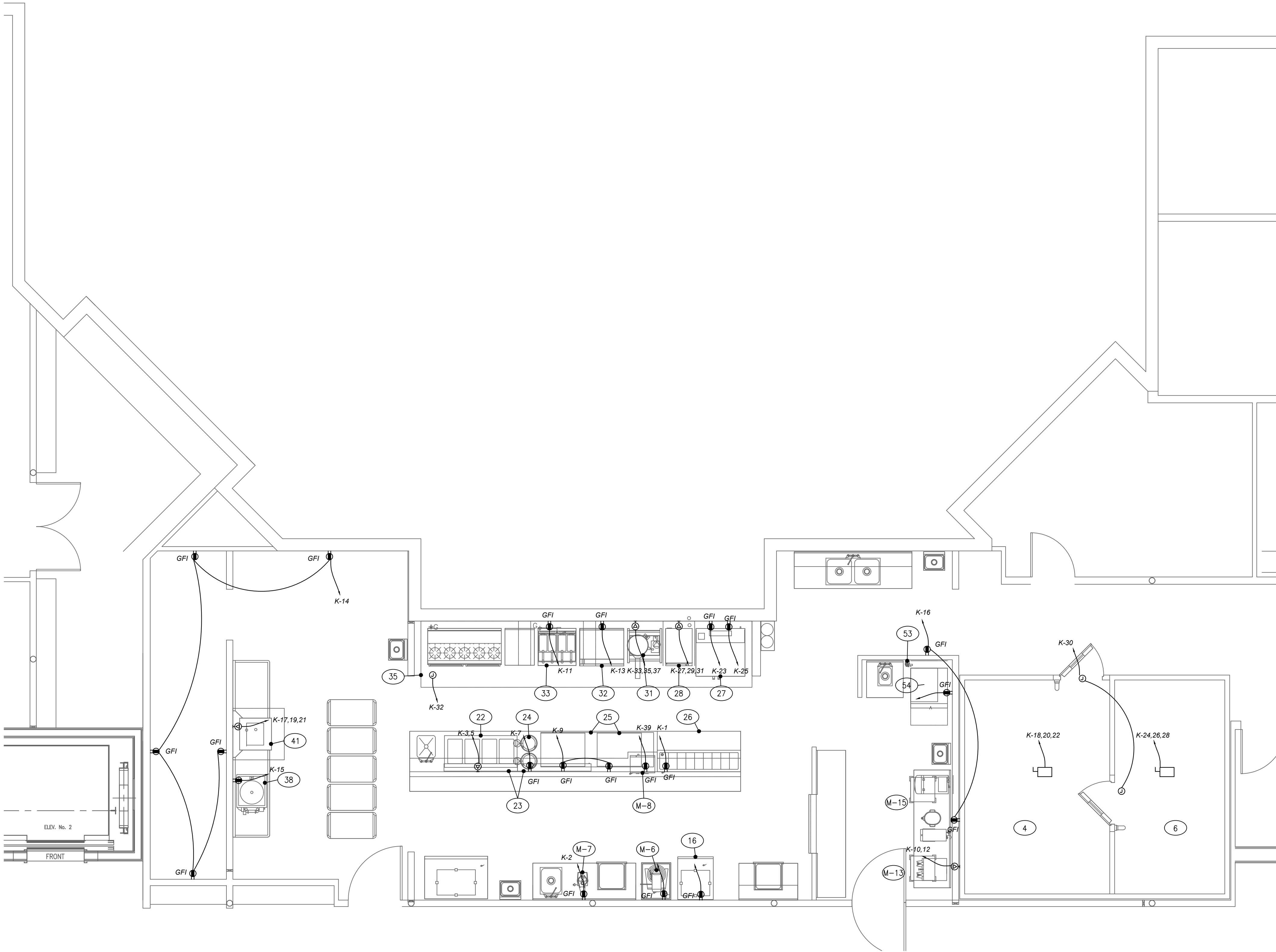
1 E12 KITCHEN POWER PLAN 1/4"=1'
